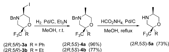
Scheme 3. Preparation of the 5-methyl-2-phenyl-2-(trifluoromethyl)morpholines ( 2R,5S )- 4a and ( 2R,5S )- 5a and the 2-ethyl-5-methyl-2-(trifluoromethyl)morpholine ( 2R,5S )- 4b .
