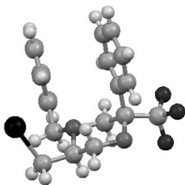
Figure 1. Molecular structure of ( 2R,5S )- 3a .
