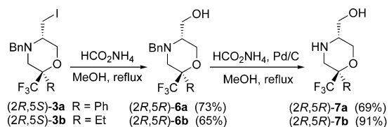
Scheme 4. Preparation of the 5-(hydroxymethyl)-2-phenyl-2-(trifluoromethyl)morpholines ( 2R,5R )- 6a , 7a and the 2-ethyl-5-(hydroxymethyl)-2-(trifluoromethyl)morpholines ( 2R,5R )- 6b , 7b .
