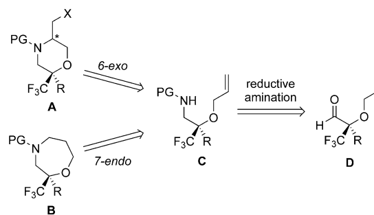
Scheme 1. Retrosynthetic scheme for the preparation of CF 3 -substituted morpholines and oxazepanes.
