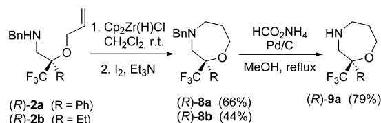
Scheme 6. Preparation of the 2-phenyl-2-(trifluoromethyl)oxazepanes ( R )- 8a , 9a and the 2-ethyl-2-(trifluoromethyl)oxazepane ( R )- 8b .
