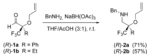
Scheme 2. Reductive amination of the aldehydes ( R )- 1a,b to the key amino ethers ( R )- 2a,b .
